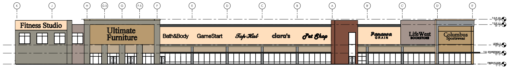
EAST ELEVATION | 1 1/16" = 1'-0"
