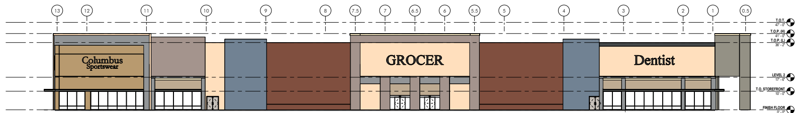
NORTH ELEVATION | 2 1/16" = 1'-0"
